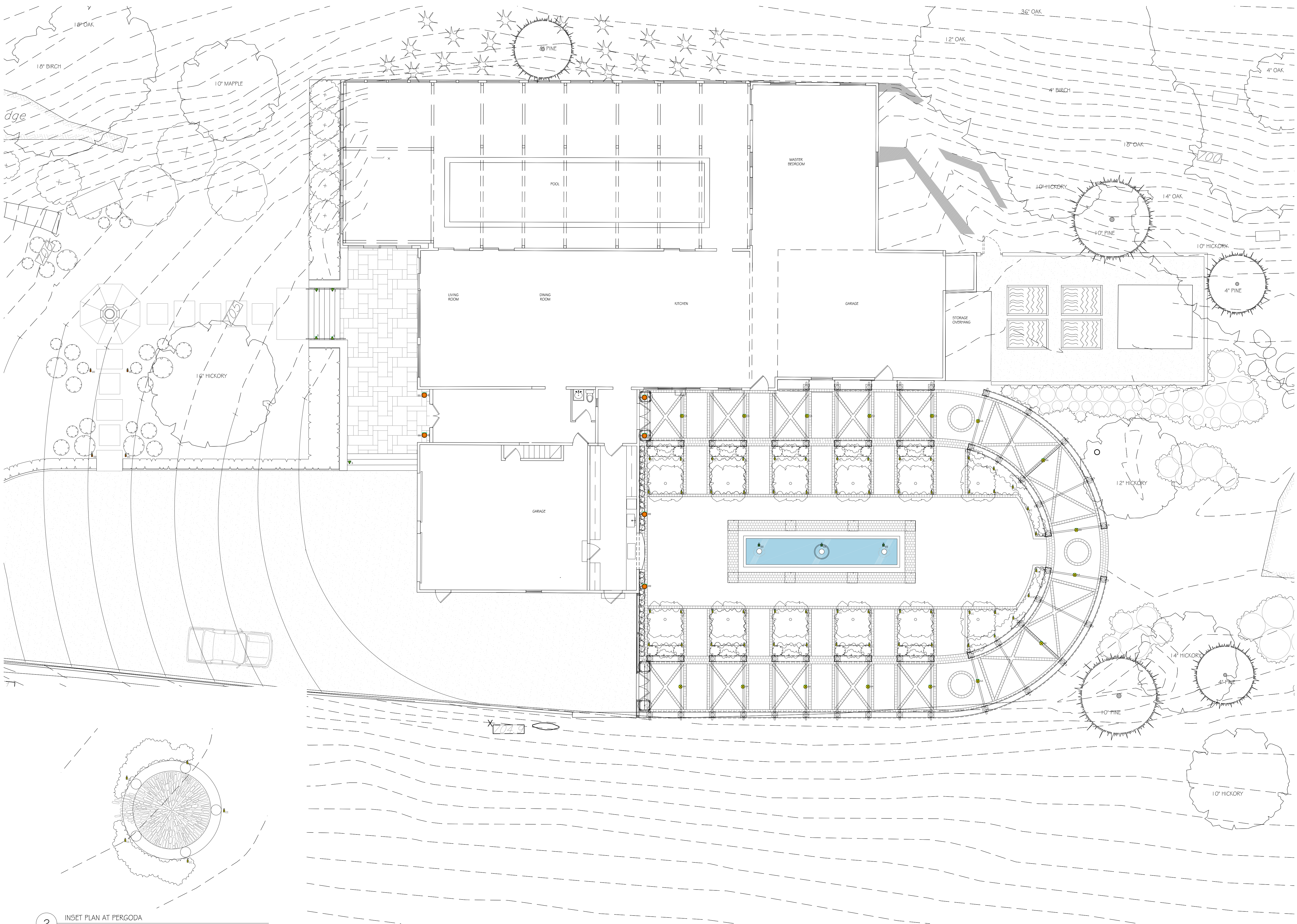
2 INSET PLAN AT PERGODA 1/8" = 1'-0"
